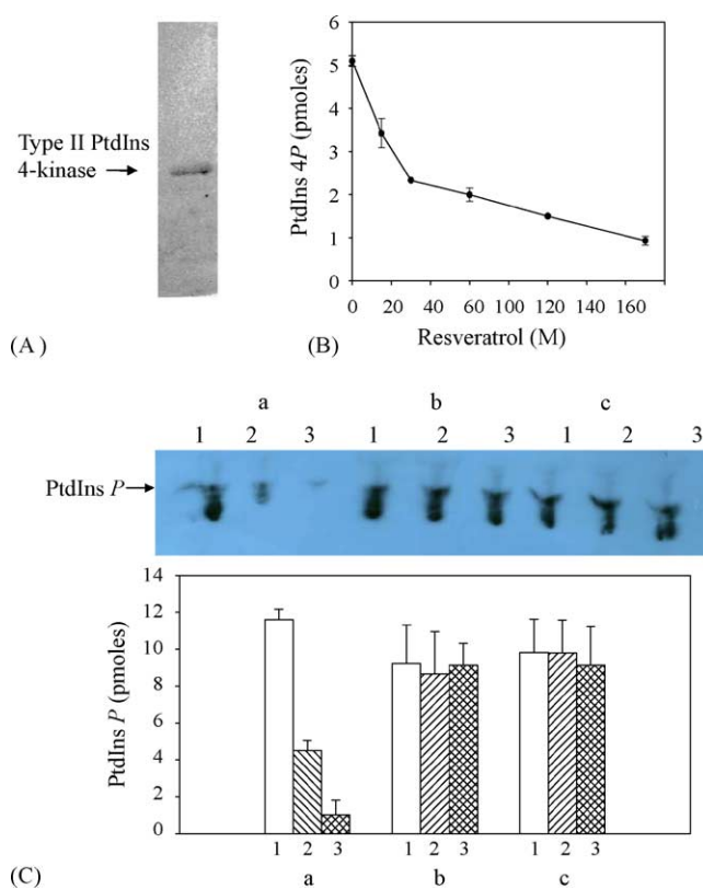
Fig. 1. Resveratrol inhibits type II PtdIns 4-kinase activity in vitro. (A) Type II PtdIns 4-kinase \beta was sub cloned and expressed in E. coli . The expressed protein was purified and analysed on SDS-PAGE. (B) The effect of resveratrol on type II PtdIns 4-kinase activity. Values are representative of four experiments. Error bars represent standard deviation (S.D.). (C) Resveratrol affects type II PtdIns 4-kinase activity but not PtdIns 3-kinase activity. Recombinant type II PtdIns 4-kinase \beta was purified from E. coli (a). Human PtdIns 3 kinases were immunoprecipitated with anti p85 (b) and anti p110 (c) subunits. All these enzymes were assayed for phosphatidylinositol kinase activities as described in Section 2. ^{32} P labeled products were analyzed on tlc and the upper panel shows the autoradiogram. Lane 1: enzyme activity in the absence of resveratrol. Lane 2: enzyme activity in presence of 50 \mu M resveratrol. Lane 3: enzyme activity in presence of 100 \mu M resveratrol. The bar diagram depicts the quantification of the data. Open bars: 0 \mu M resveratrol, hatch bars: 50 \mu M resveratrol, and cross-bars: 100 \mu M resveratrol. The values are mean of three experiments \pm S.E. The P value is \leq 0.002 (one-way ANOVA).
