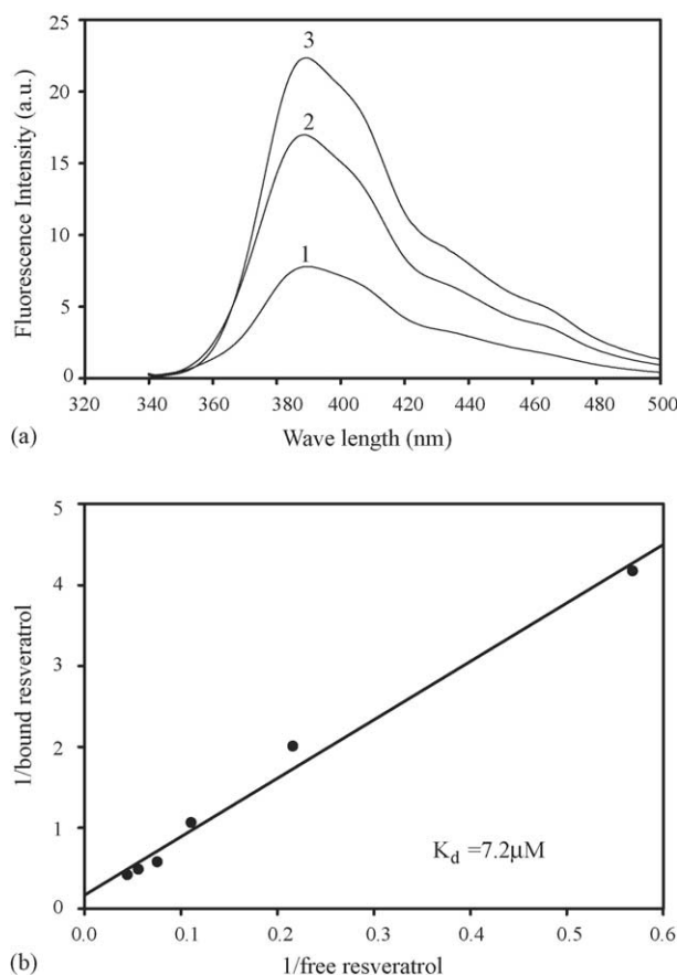
Fig. 2. Type II PtdIns 4-kinase \beta directly binds to resveratrol. Binding of resveratrol to type II PtdIns 4-kinase was determined by fluorescence spectroscopy. (A) Resveratrol (5 \mu M) was incubated with type II PtdIns 4-kinase \beta as described in experimental procedures, and the emission spectra were collected after excitation at 320 nm. (1) Free resveratrol (5 \mu M); (2) resveratrol (5 \mu M) incubated with 5 \mu M PtdIns 4-kinase; and (3) resveratrol (5 \mu M) with 10 \mu M PtdIns 4-kinase. (B) Double reciprocal plot for the binding of resveratrol to type II PtdIns 4-kinase \beta . The fluorescence intensity at 389 nm was used to calculate the concentration of bound and free resveratrol. The experiment is representative of three experiments.
