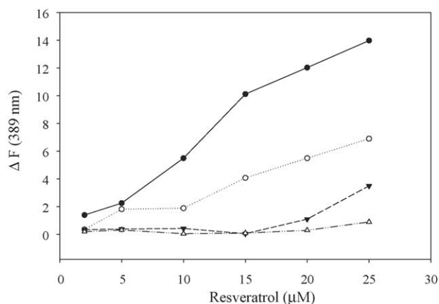
Fig. 3. Resveratrol competes with phosphatidylinositol binding. Type II PtdIns 4-kinase (5 \mu M) was incubated with increasing concentrations of resveratrol (2–25 \mu M) in presence of varying concentrations of phosphatidylinositol. Fluorescence intensity at 389 nm was measured to calculate the increase in resveratrol fluorescence upon protein binding. Increase in fluorescence was measured in absence of phosphatidylinositol (●), in presence of 2 \mu M phosphatidylinositol (○), 5 \mu M PtdIns (△) and 20 \mu M PtdIns (▲). Values are representative of four experiments.
